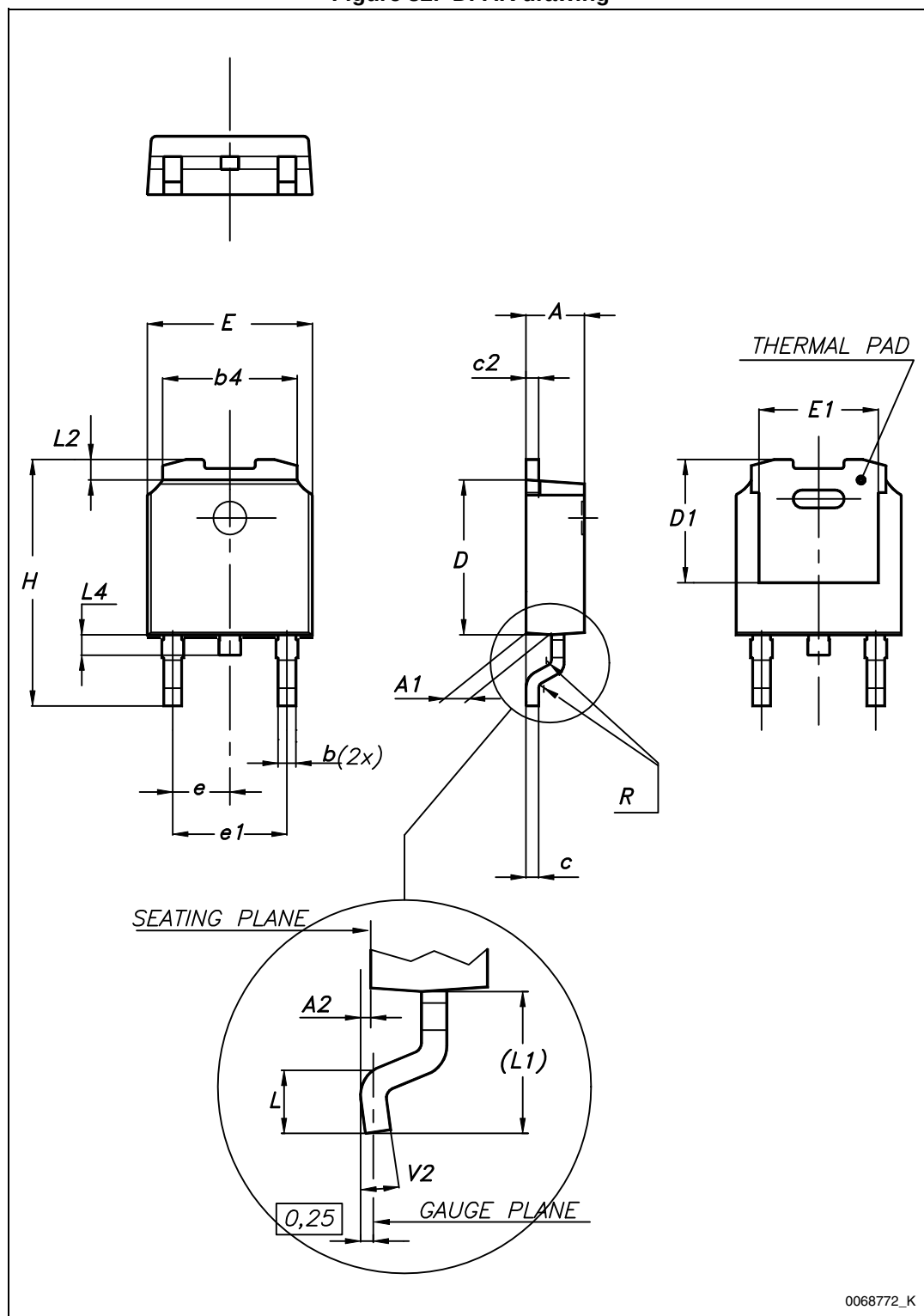
Figure 32. DPAK drawing
