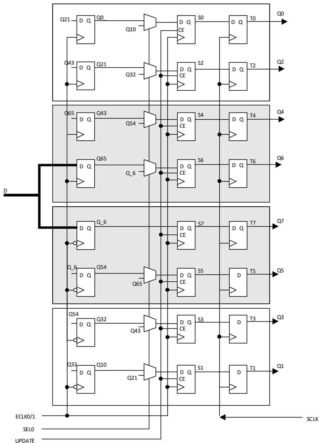
Figure 2.16. Input Gearbox
