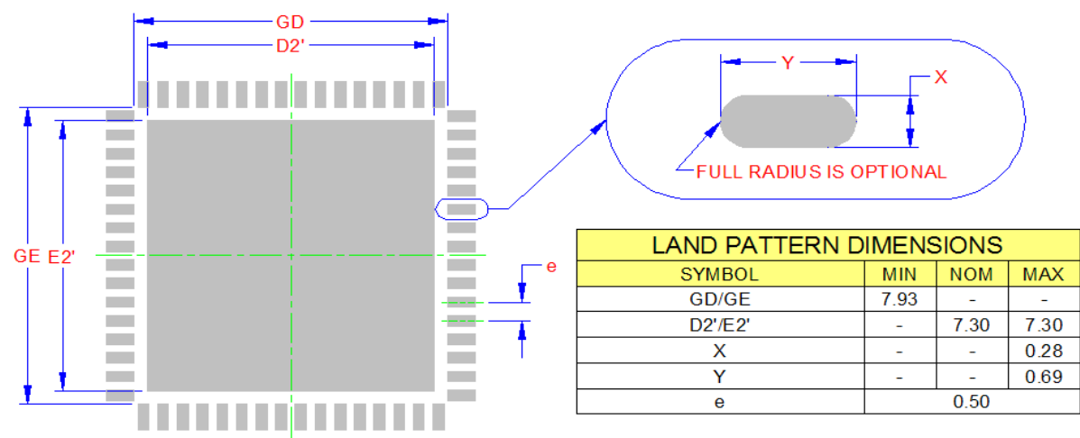
FIGURE 5-2: LAN9512/LAN9512I RECOMMENDED PCB LAND PATTERN
