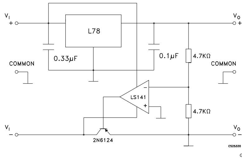
Figure 17. Split power supply ( \pm 15V - 1A )
