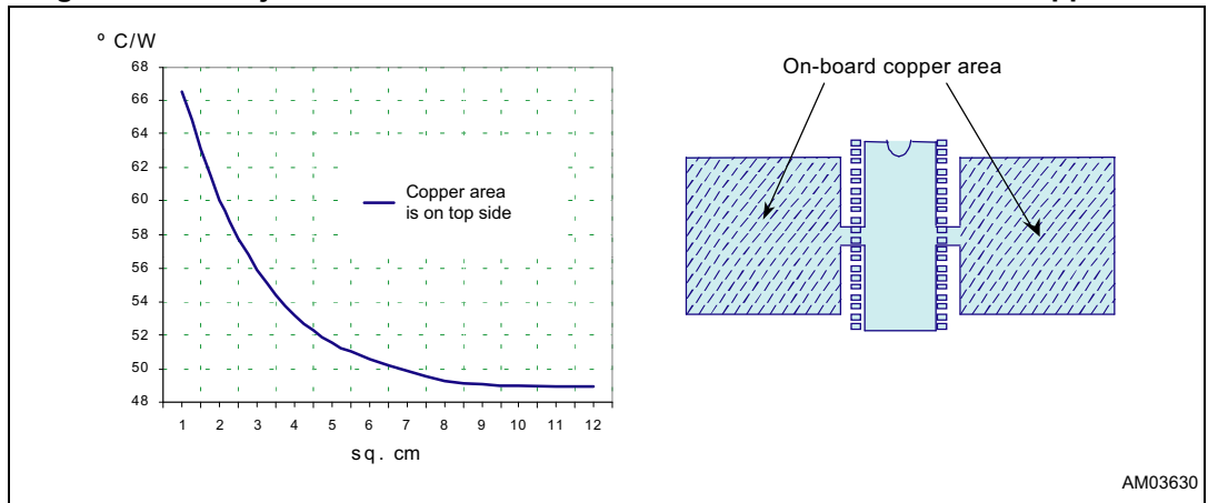
Figure 22. SO24 junction ambient thermal resistance versus on-board copper area
