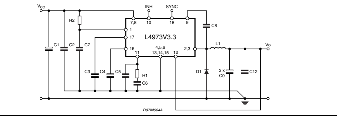
Figure 8. Application circuit (see Figure 4 part list)
