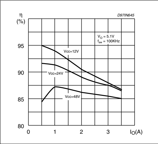
Figure 28. Efficiency vs. output current (see Figure 7)
