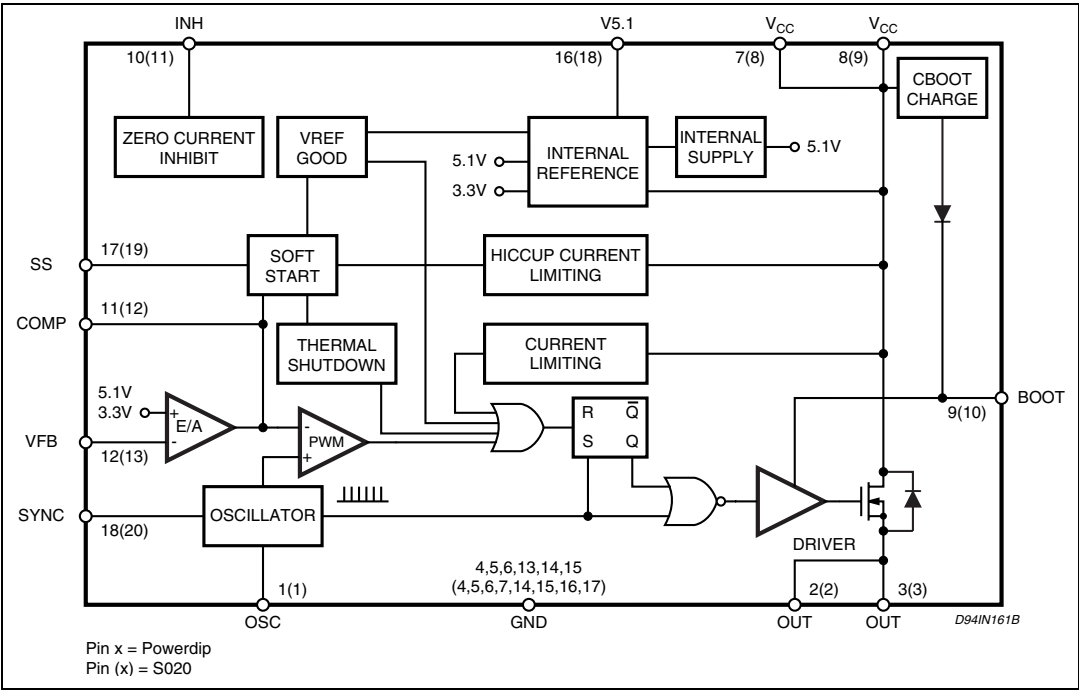
Figure 2. Block diagram
