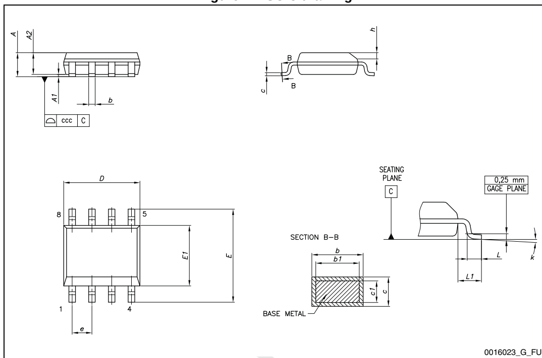
Figure 12. SO-8 drawing
