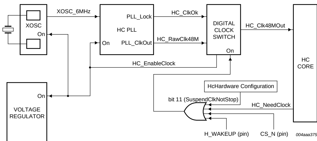
Fig 28. ISP1160/01 suspend and resume clock scheme.
