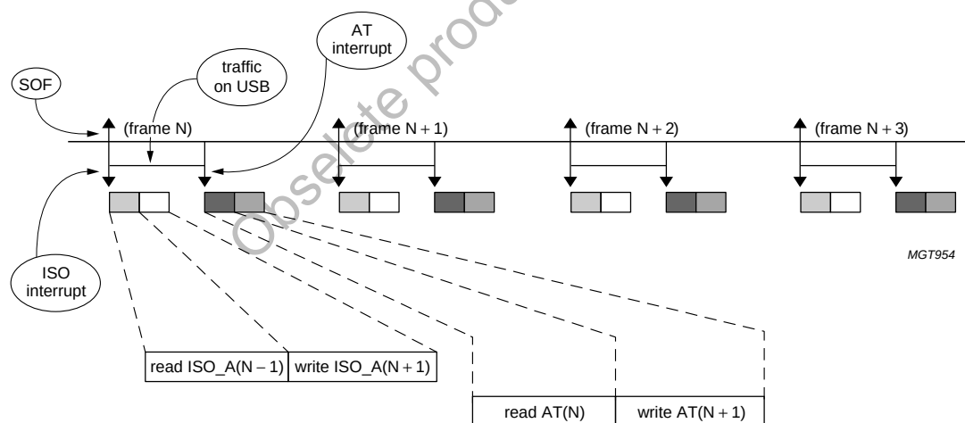
Fig 21. HC time domain behavior: example 1.
