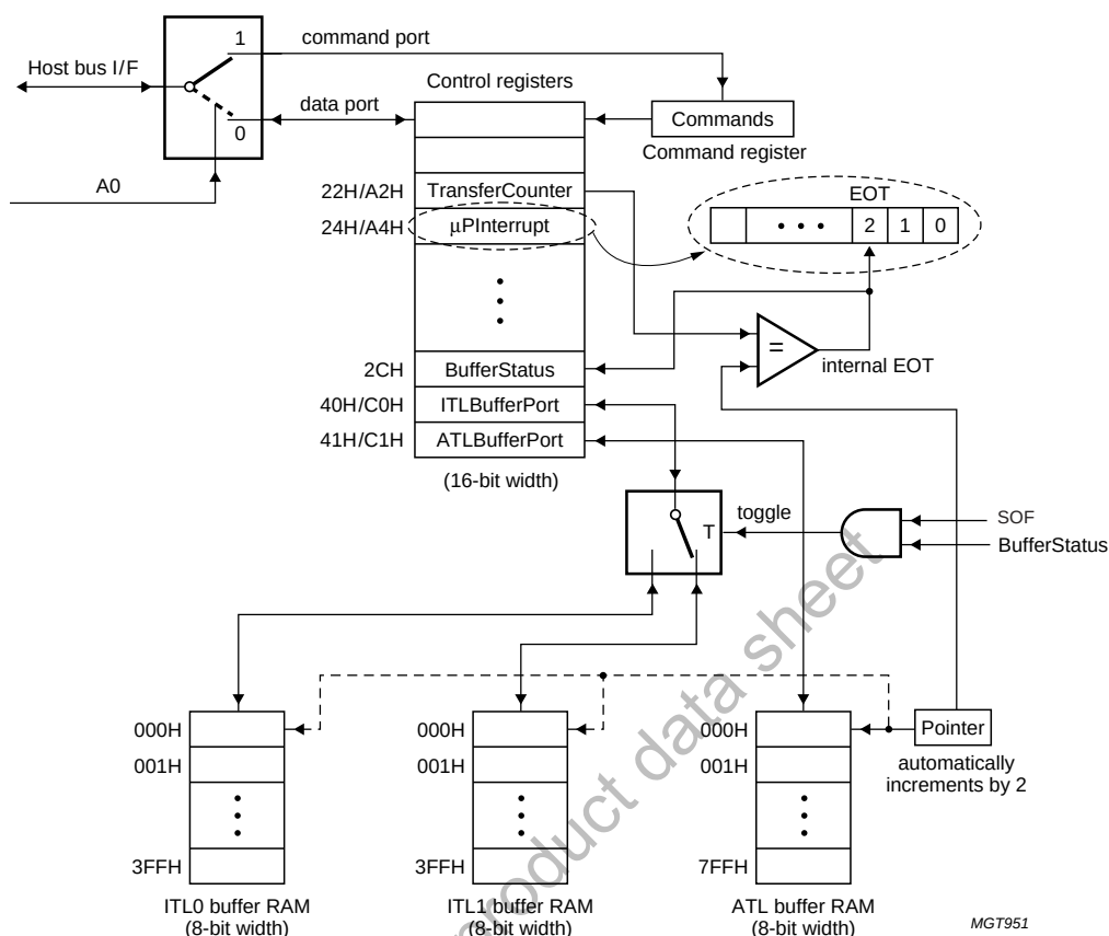
Fig 20. PIO access to internal FIFO buffer RAM.
