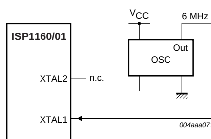
Fig 32. Oscillator circuit using external oscillator.
