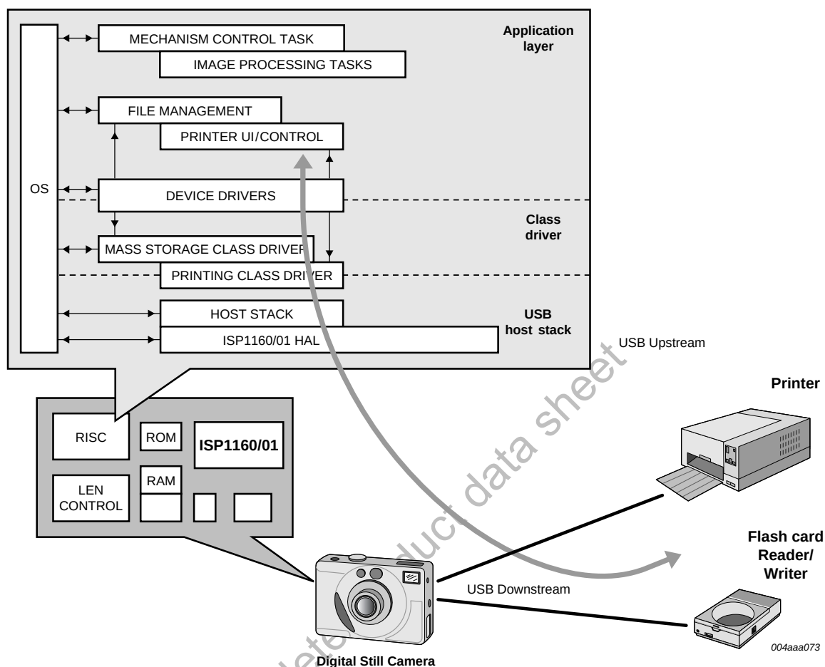
Fig 41. The ISP1160/01 software model for DSC application.
