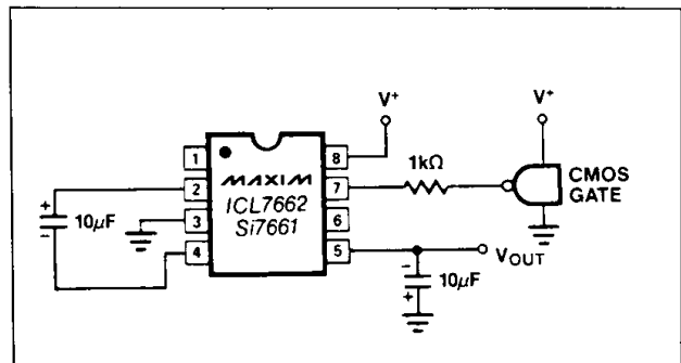
Figure 4. External Clocking
