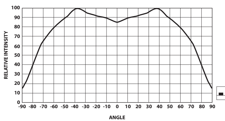
Figure 6. Relative intensity vs. angle for HSMx-C120.
