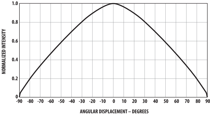
Figure 8: Radiation Pattern
