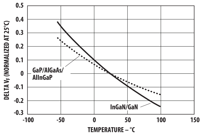
Figure 7: Forward Voltage Shift vs. Temperature
