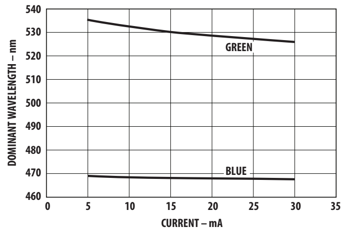
Figure 6: Dominant Wavelength vs. Forward Current (InGa Devices)
