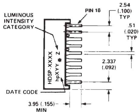
TOP END VIEW R, S
