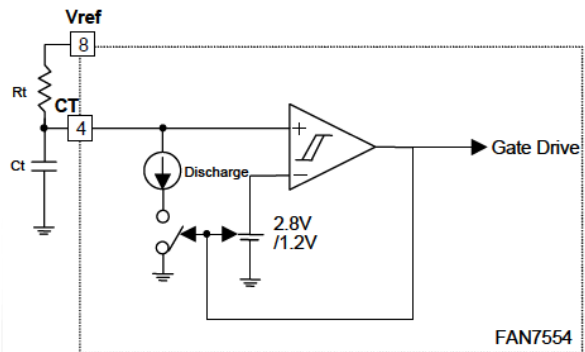
Figure 17. Oscillator Circuit
