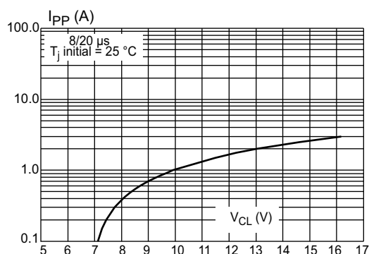
Figure 5. Clamping voltage versus peak pulse current (typical values, 8/20 μs waveform)
