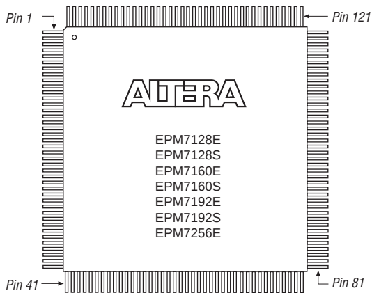
160-Pin PQFP
