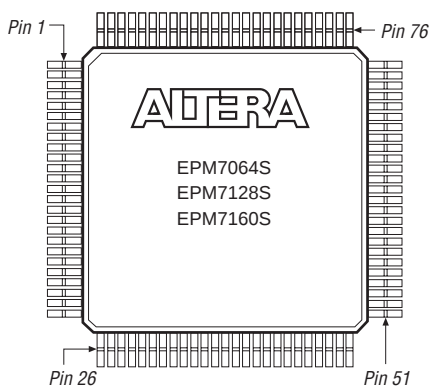
100-Pin TQFP
