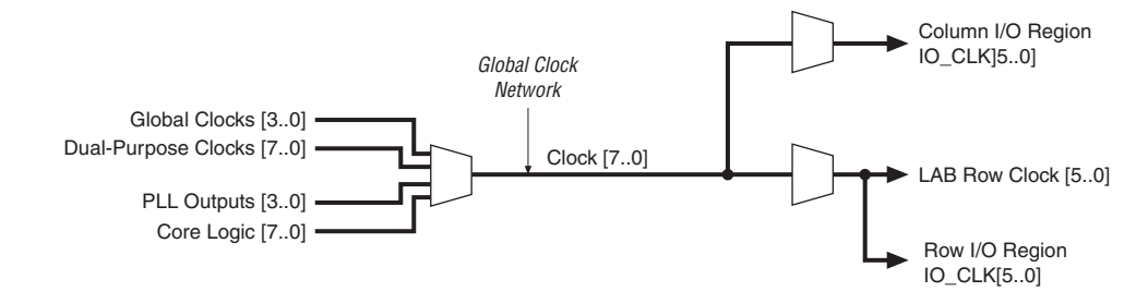
Figure 2-23. Global Clock Network Multiplexers
