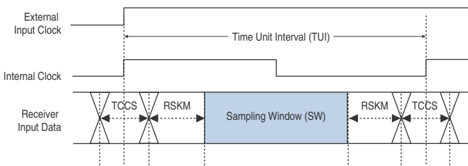
Figure 9–9. High-Speed I/O Timing Diagram
