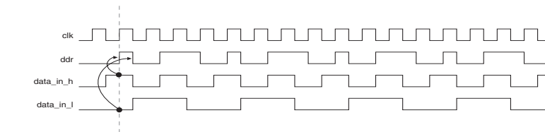
Figure 10–4. Double Data Rate Output Waveforms
