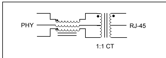
FIGURE 2-6: ALTERNATE TX CHOKER TOPOLOGY
