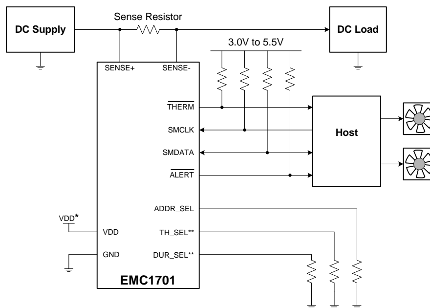
Figure 4.1 EMC1701 System Diagram
