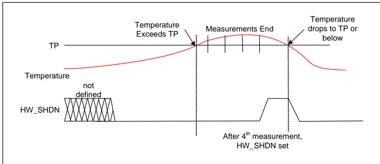
Figure 5.5 HW_SHDN Operation
