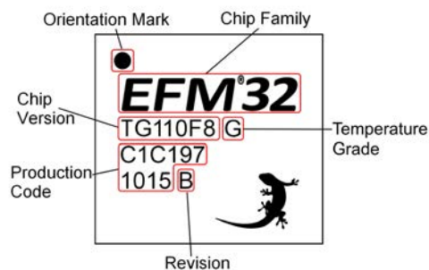
Figure 6.1. Example Chip Marking (top view)
