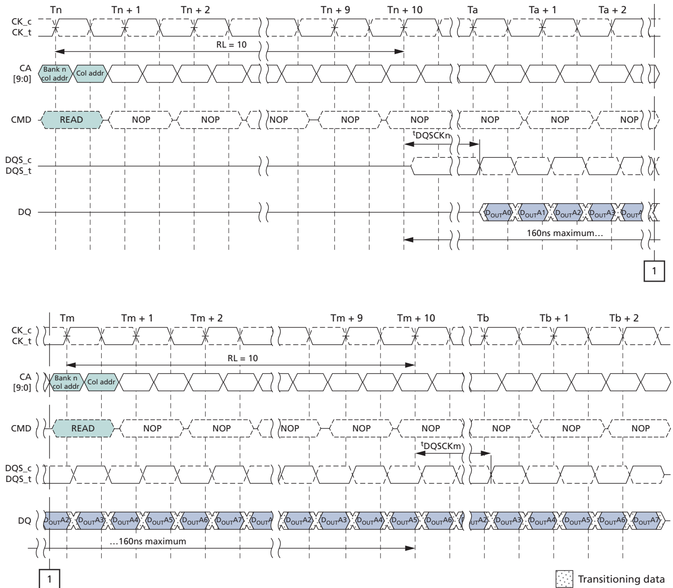
Figure 22: t_{DQSCKDS} Timing
