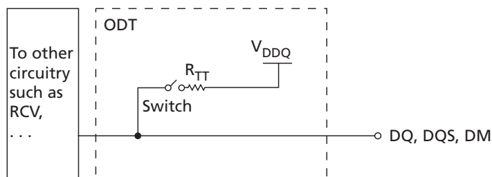
Figure 52: Functional Representation of On-Die Termination
