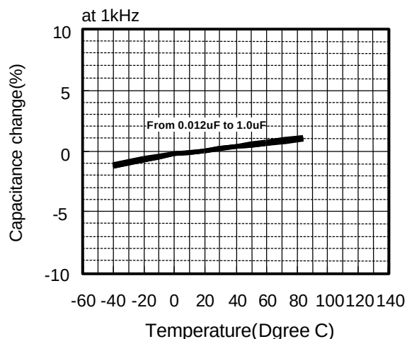
Temperature Characteristics
