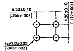
Through-hole
