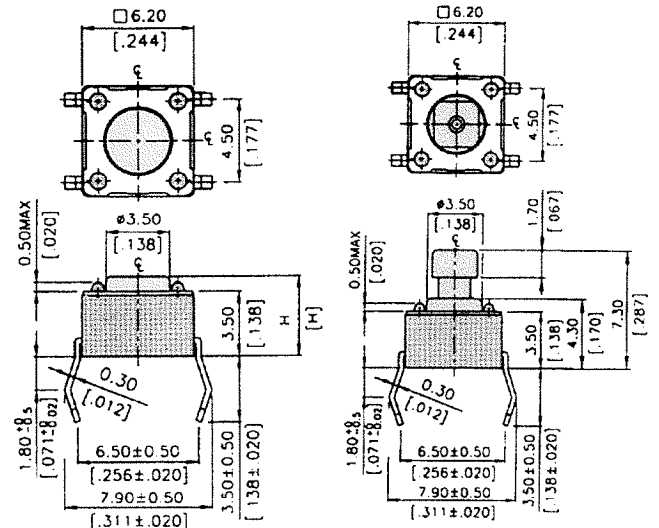
Through-hole
