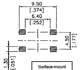
Surface-mount
