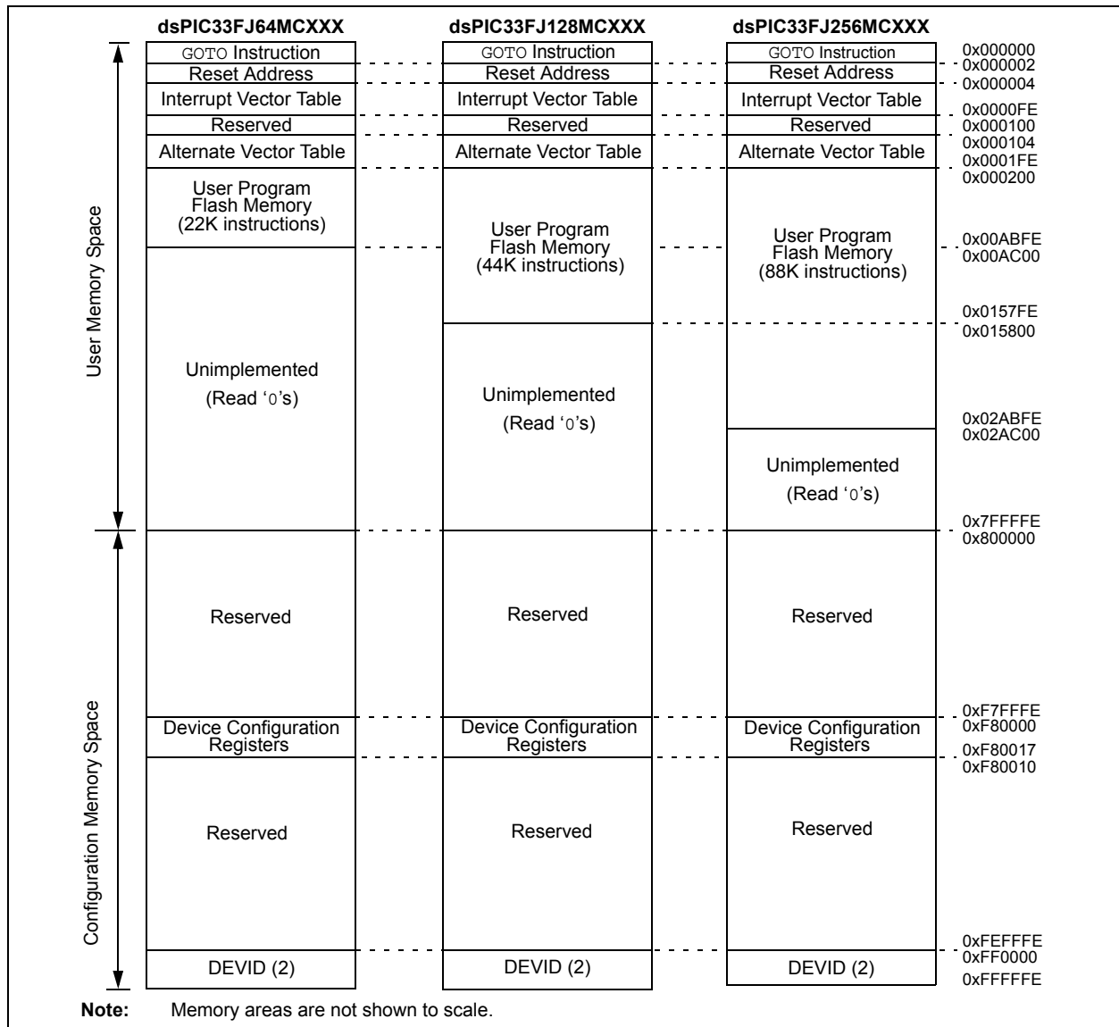
FIGURE 4-1: PROGRAM MEMORY MAP FOR dsPIC33FJXXMXX06/X08/X10 DEVICES
