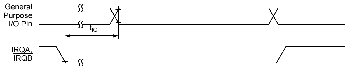
Figure 3-16 External Level-Sensitive Interrupt Timing
