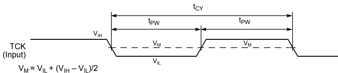
Figure 3-29 Test Clock Input Timing Diagram
