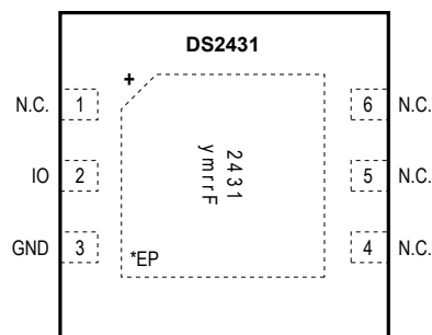
TDFN (3mm x 3mm) *EXPOSED PAD
