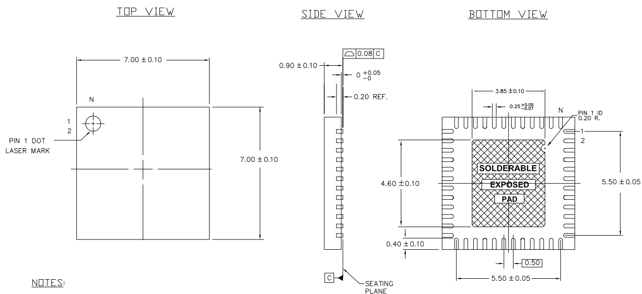
Figure 2. 48-pin QFN 7x7 mm LT48E (Sawn)
