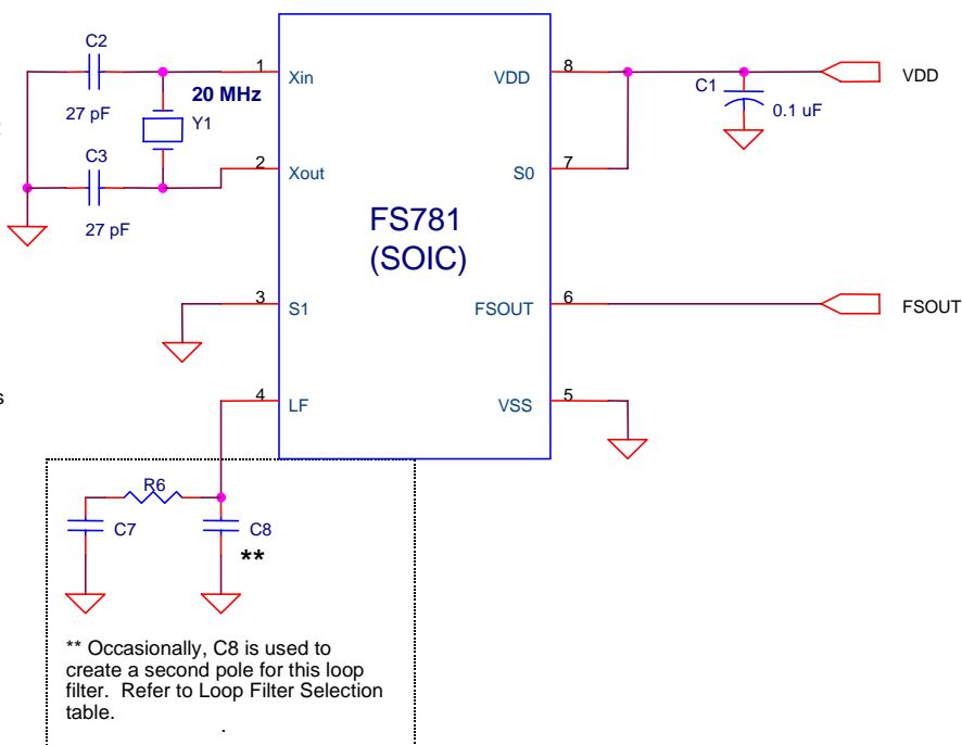
Figure 5. FS781 Schematic
