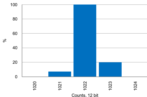
Figure 11-39. SAR ADC Noise Histogram, 1 mps, External Reference
