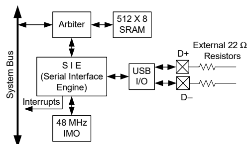
Figure 7-14. USB
