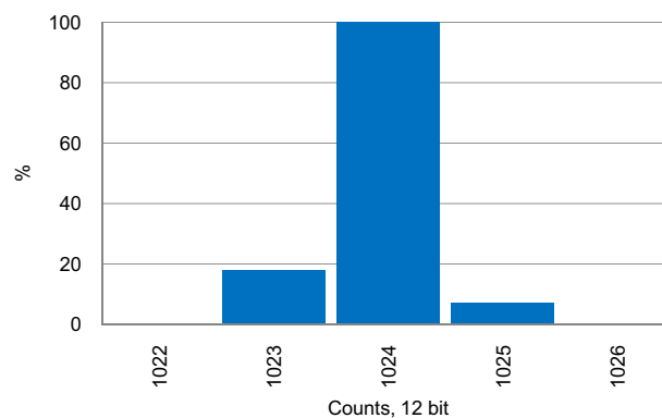
Figure 11-38. SAR ADC Noise Histogram, 1 mps, Internal Reference Bypassed
