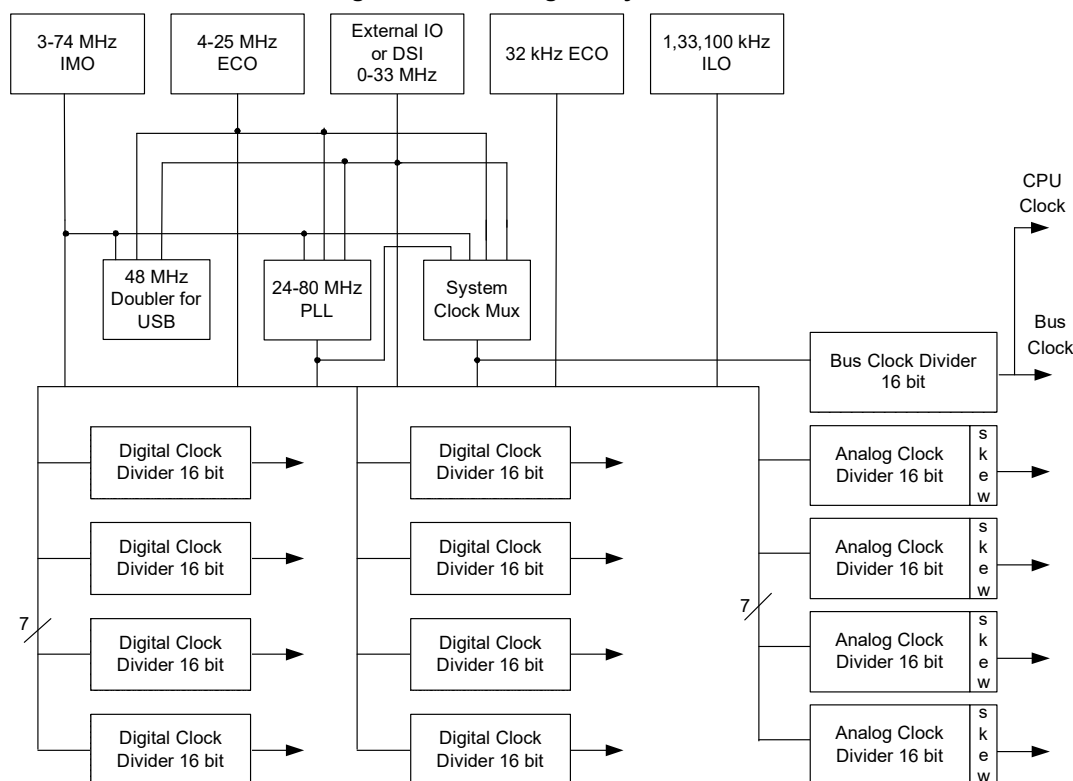
Figure 6-1. Clocking Subsystem
