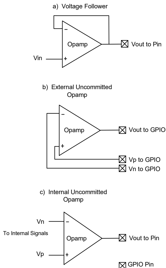
Figure 8-8. Opamp Configurations
