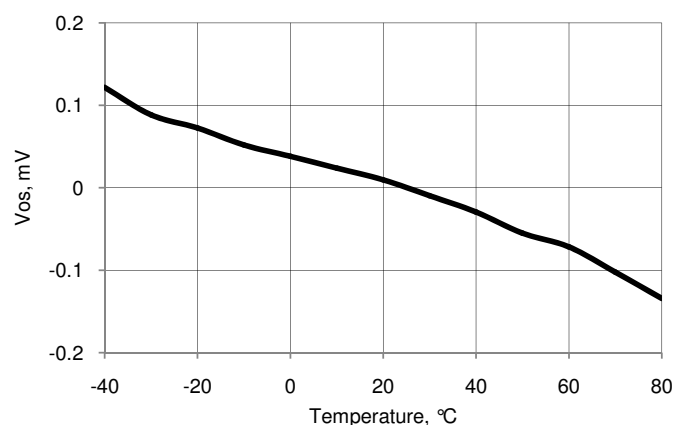
Figure 11-26. Opamp V_{os} vs Temperature, V_{DDA} = 5\text{ V}
