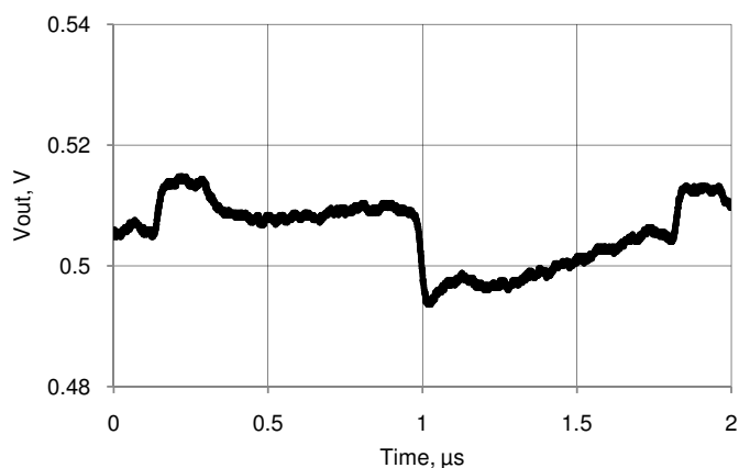
Figure 11-65. VDAC Voltage Noise, 1 V Mode, Fast Mode, V_{DDA} = 5 V
