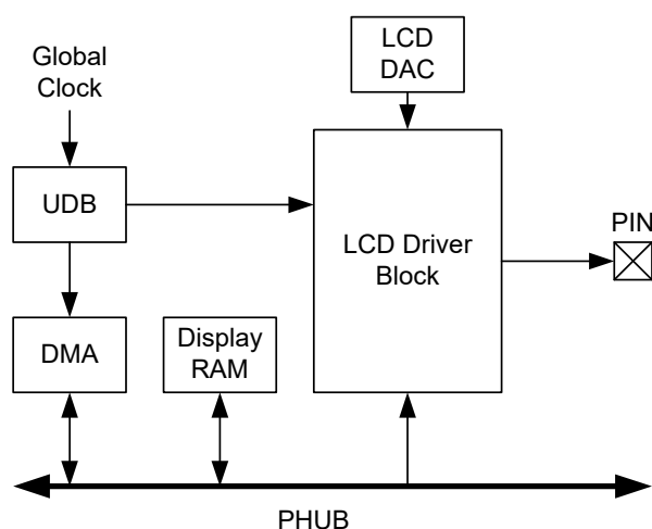
Figure 8-11. LCD System
