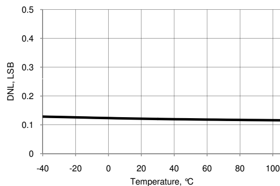
Figure 11-57. VDAC DNL vs Temperature, 1 V Mode
