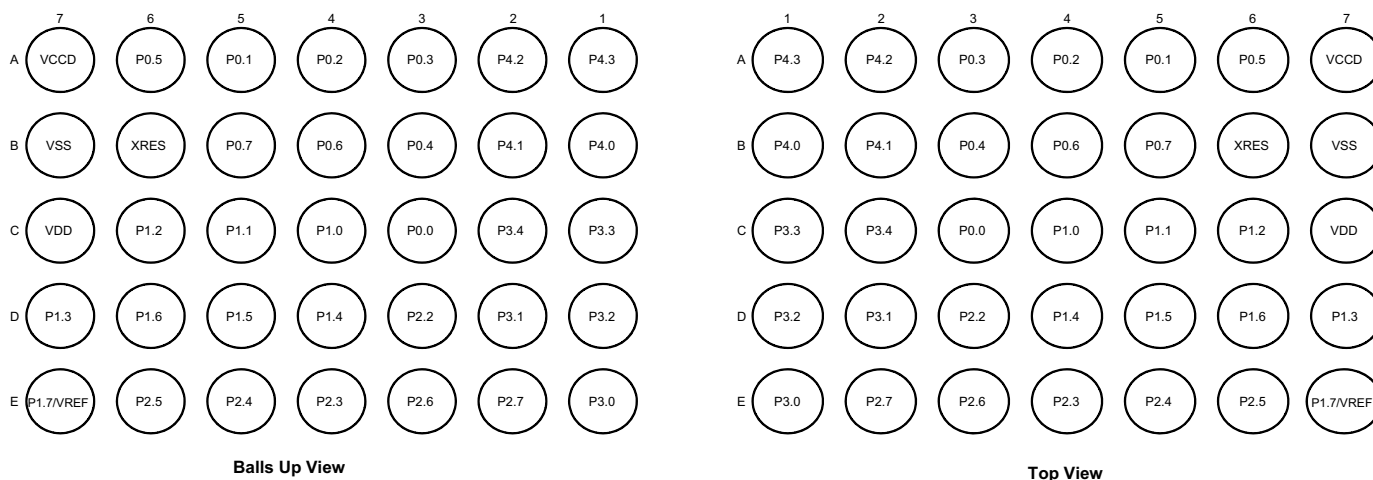
Figure 8. 35-Ball WLCSP
