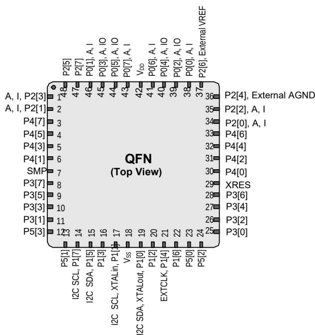
Figure 7. CY8C29666 48-Pin PSoC Device
