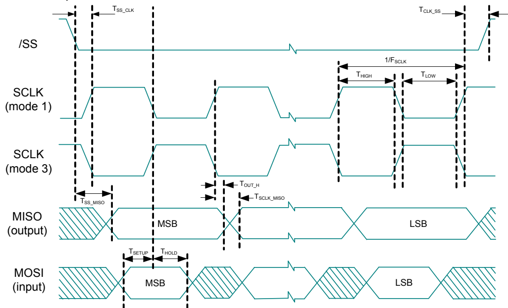
Figure 12. SPI Slave Mode 1 and 3
