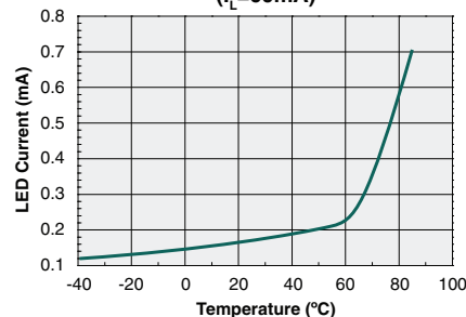
Typical I_F for Switch Operation ( I_L=60\text{mA} )
