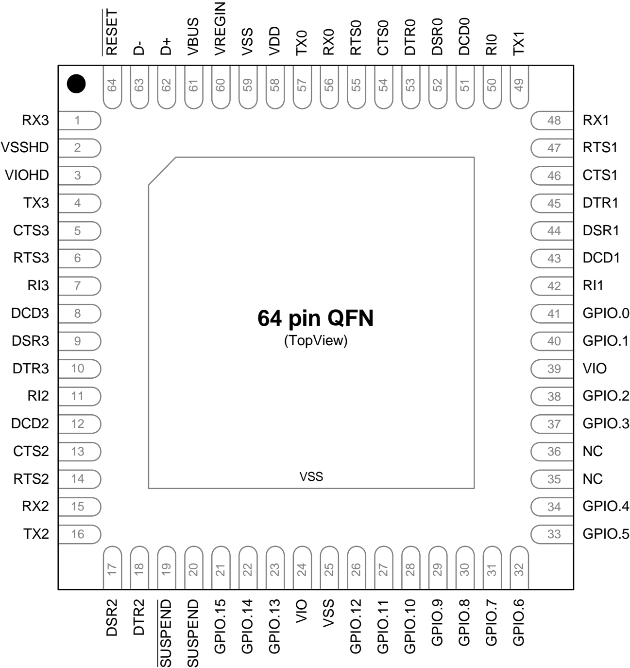
Figure 2. QFN-64 Pinout
