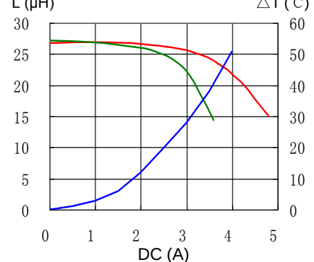
12. CDRH125NP-270MC
