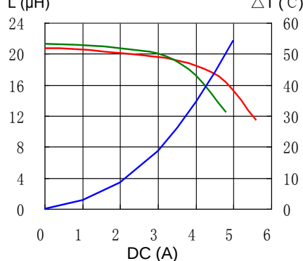
11. CDRH125NP-220MC
