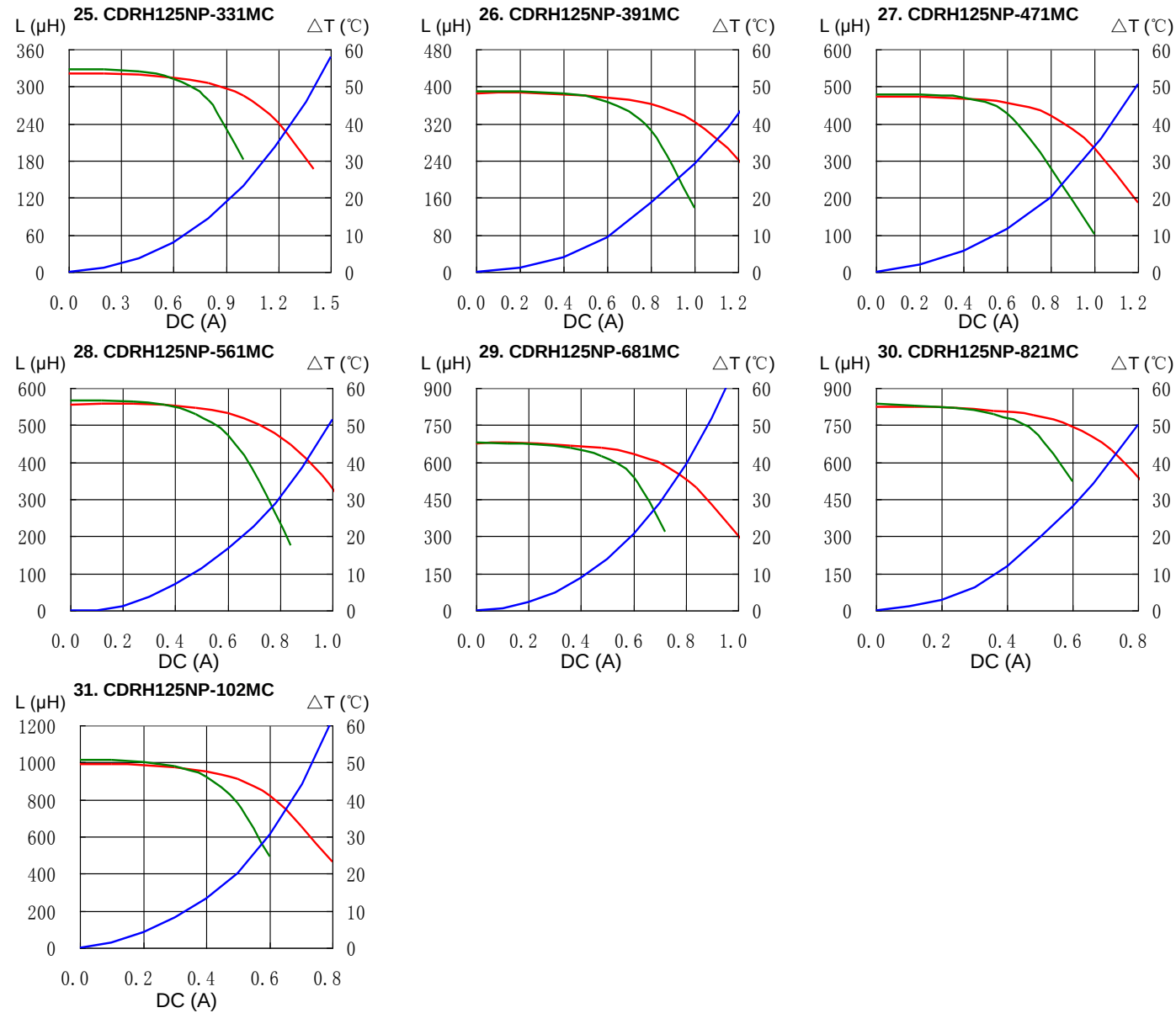
Saturation Current & Temperature Rise Graph
