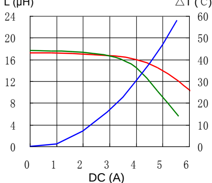
10. CDRH125NP-180MC
