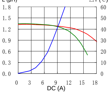
4. CDRH125NP-4R4NC
