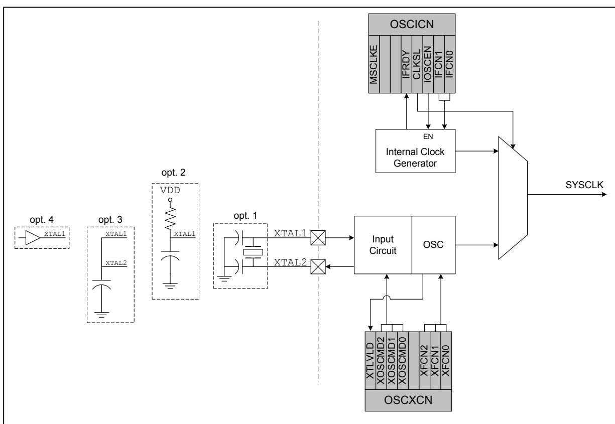
Figure 13.1. Oscillator Diagram
