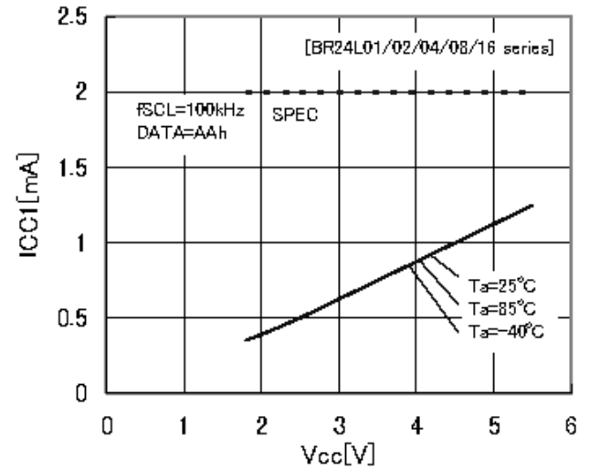
Figure 11. Current consumption at WRITE action ICC1 (fsc=100kHz)
