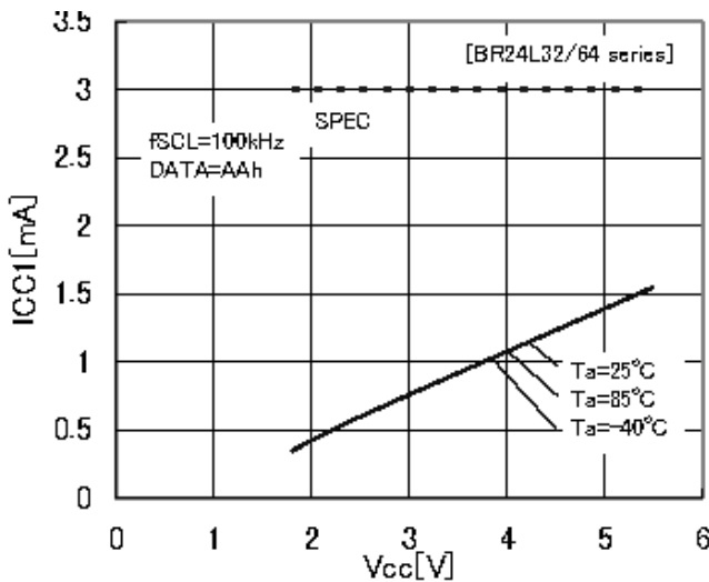
Figure 12. Current consumption at WRITE action ICC1 (fsc=100kHz)
