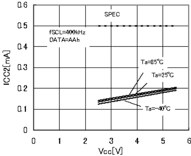
Figure 10. Current consumption at READ action ICC2 (fsc=400kHz)
