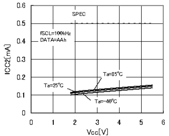
Figure 13. Current consumption at READ action ICC2 (fsc=100kHz)
