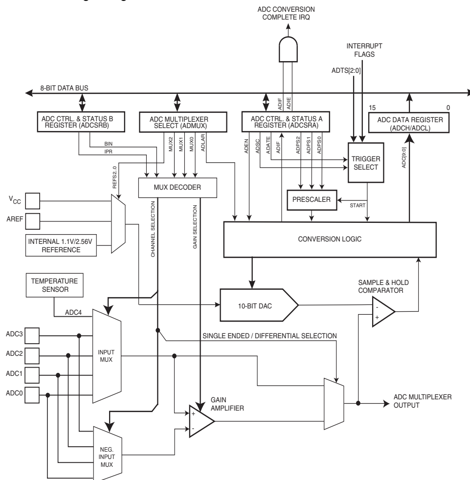
Figure 18-1. Analog to Digital Converter Block Schematic
