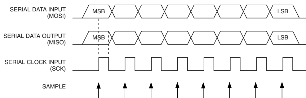
Figure 21-2. Serial Programming Waveforms
