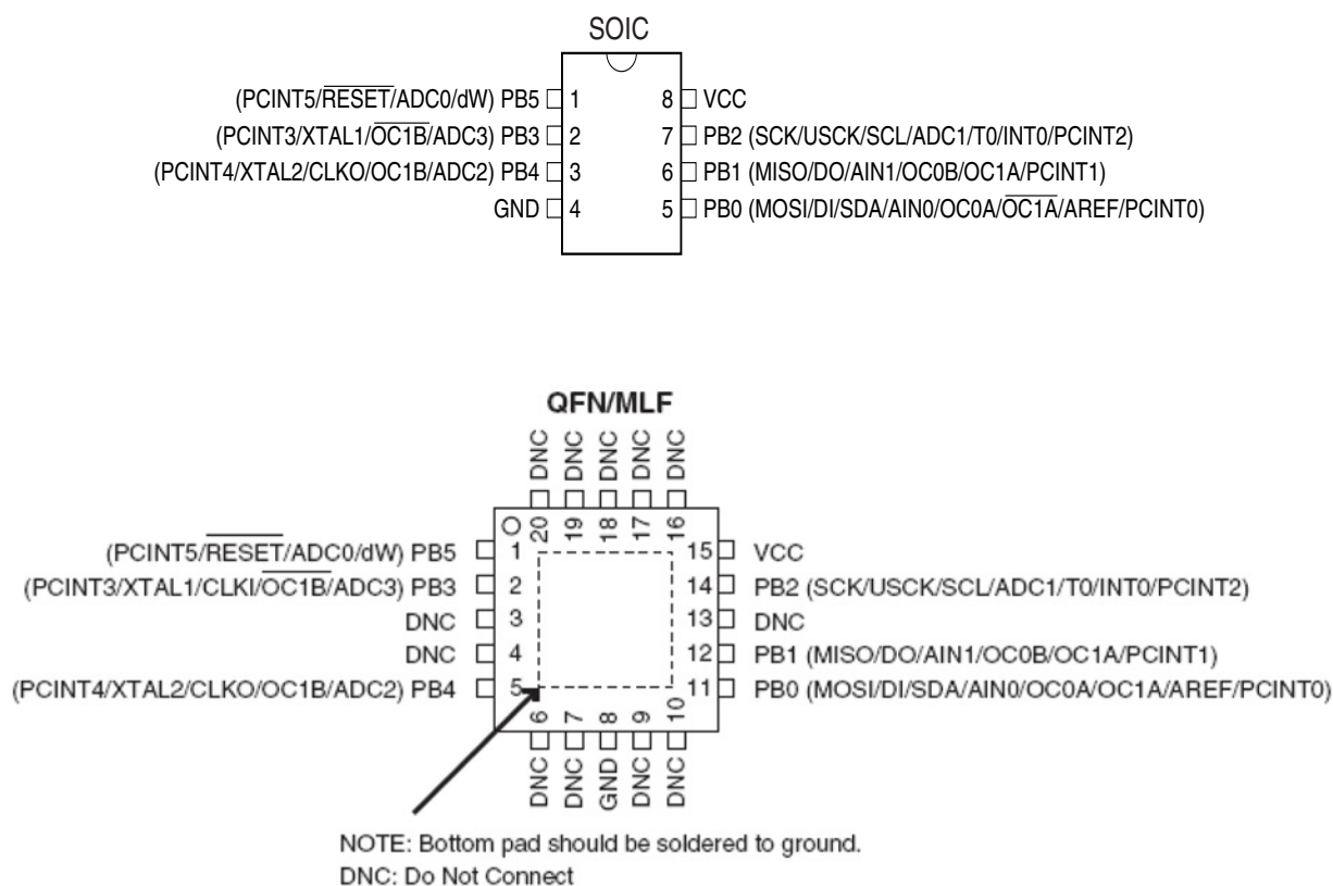
Figure 1-1. Pinout ATtiny25/45/85
