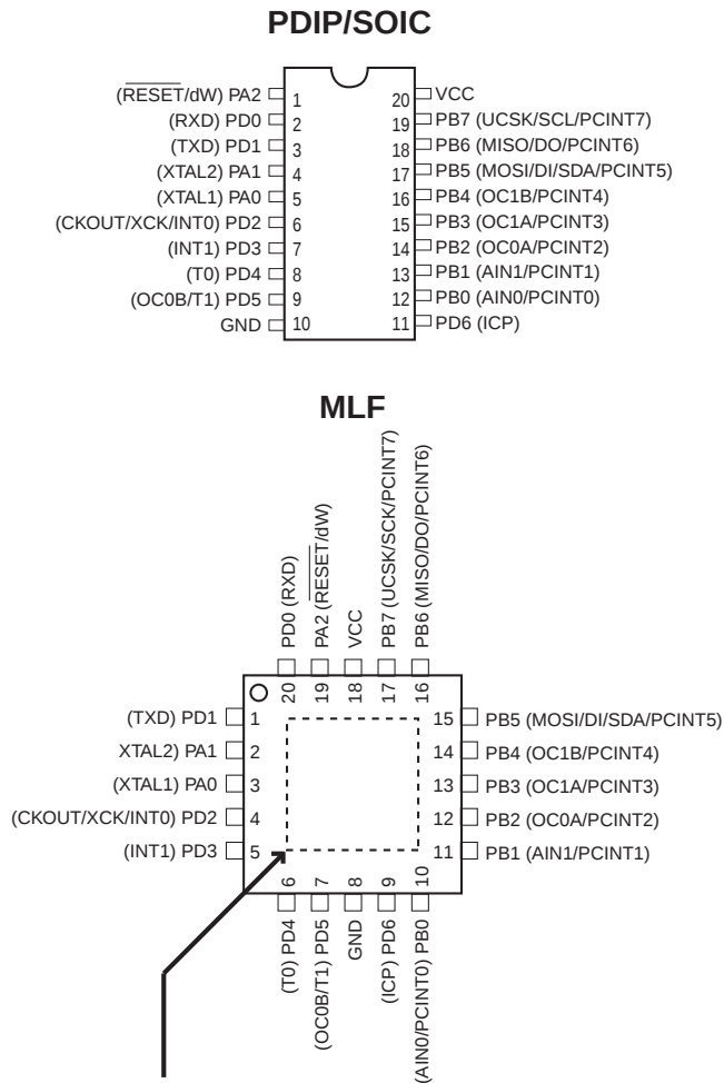
Figure 1. Pinout ATtiny2313
