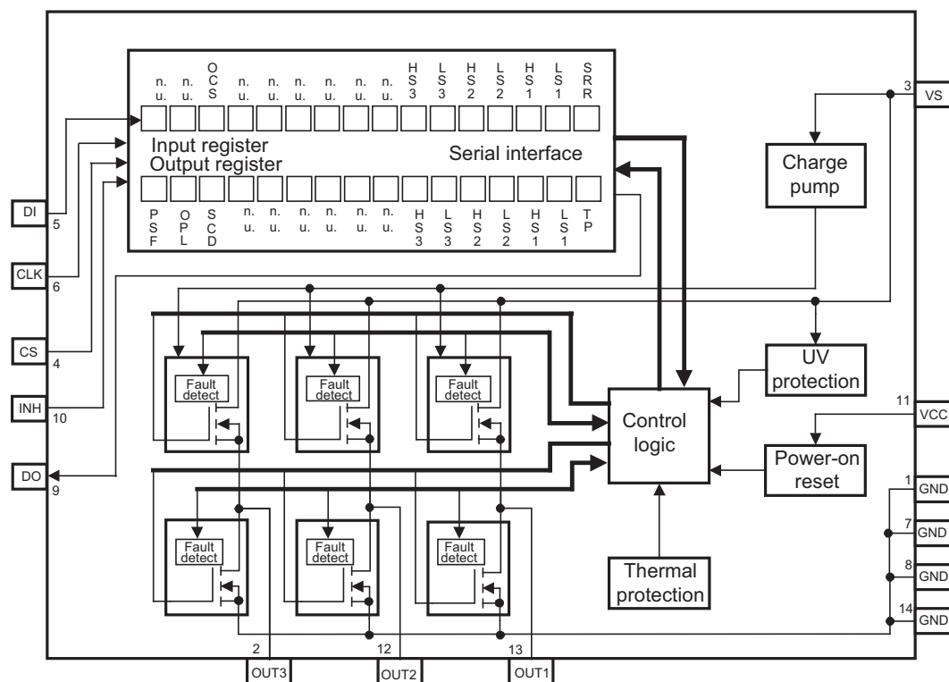
Figure 1-1. Block Diagram
