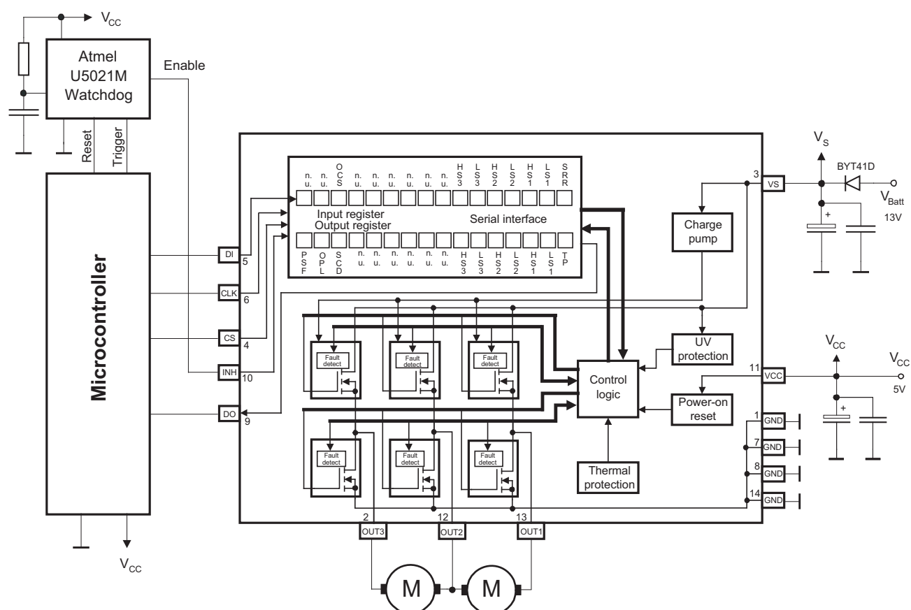
Figure 10-1. Application Circuit
