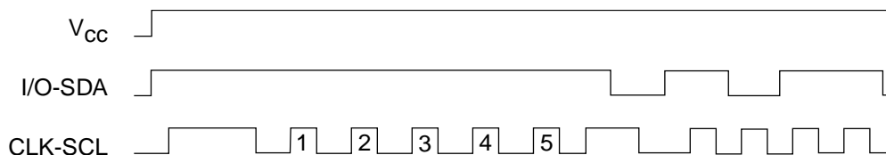
Figure 11. Start-up Sequence
