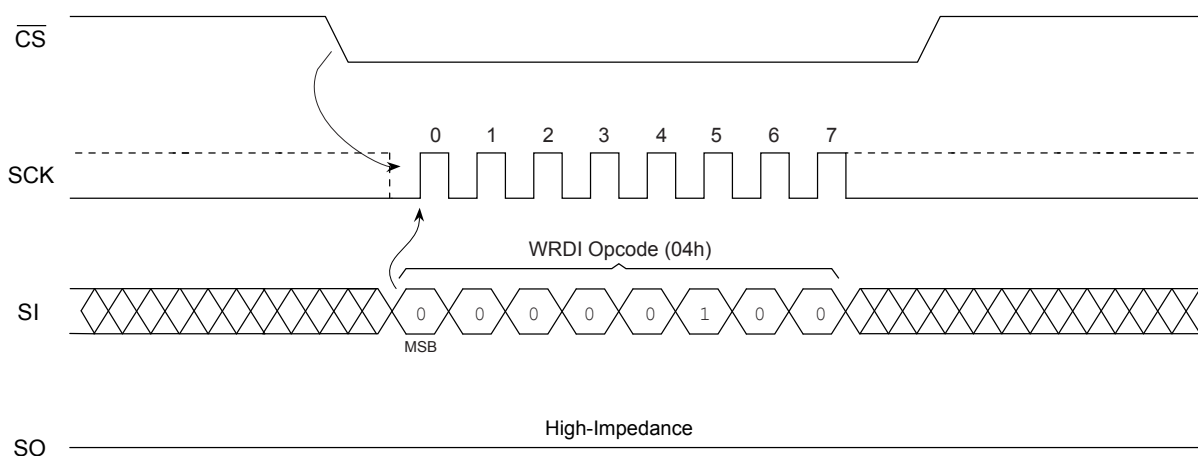
Figure 6-3. \overline{WRDI} Timing
