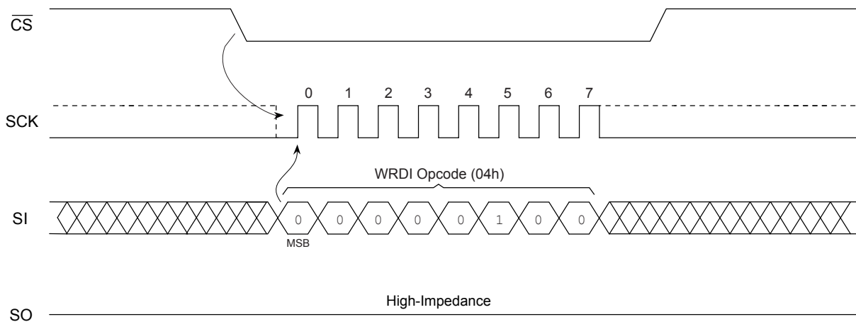
Figure 6-3. \overline{WDI} Timing
