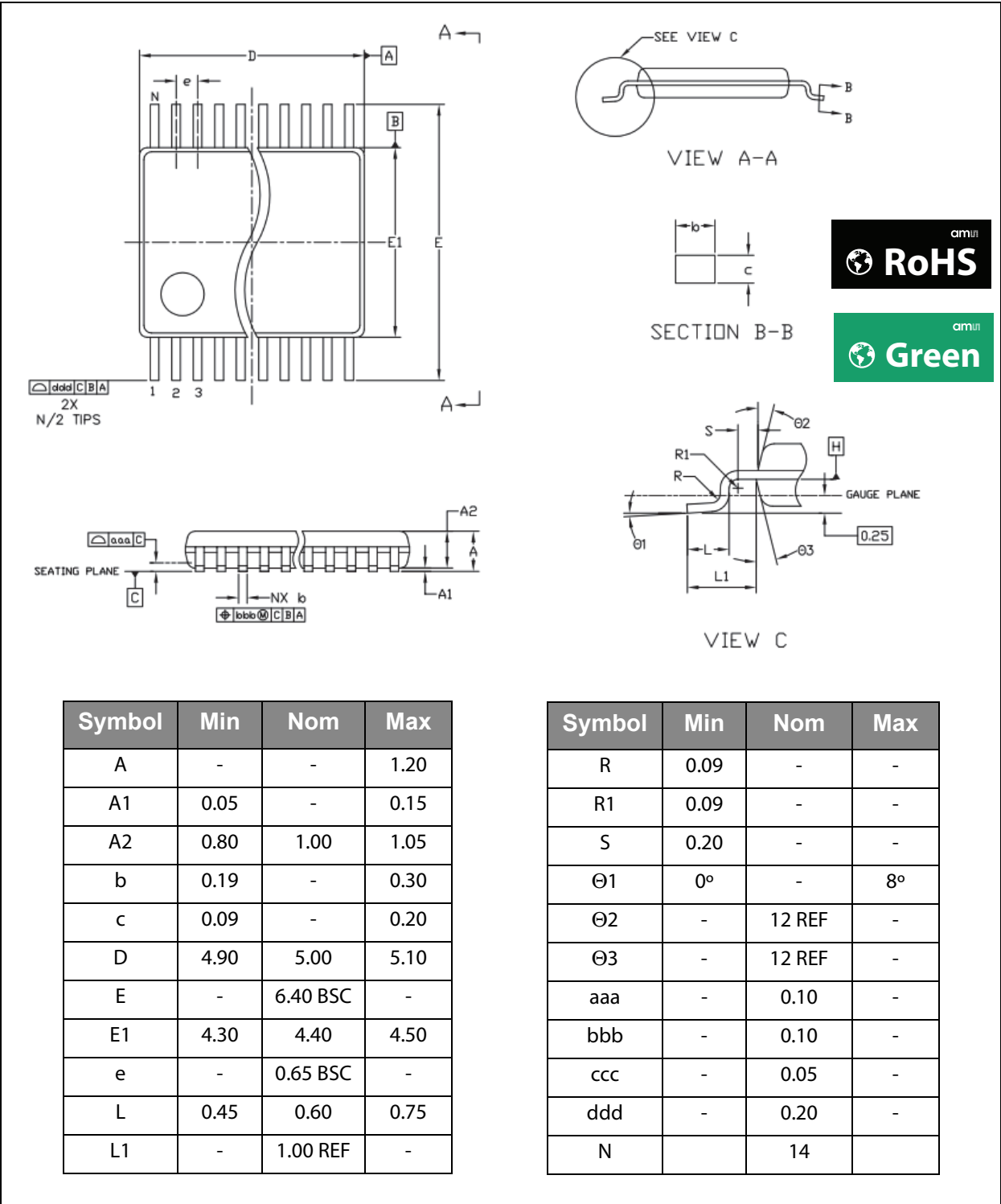
Figure 40: Package Outline Drawing
