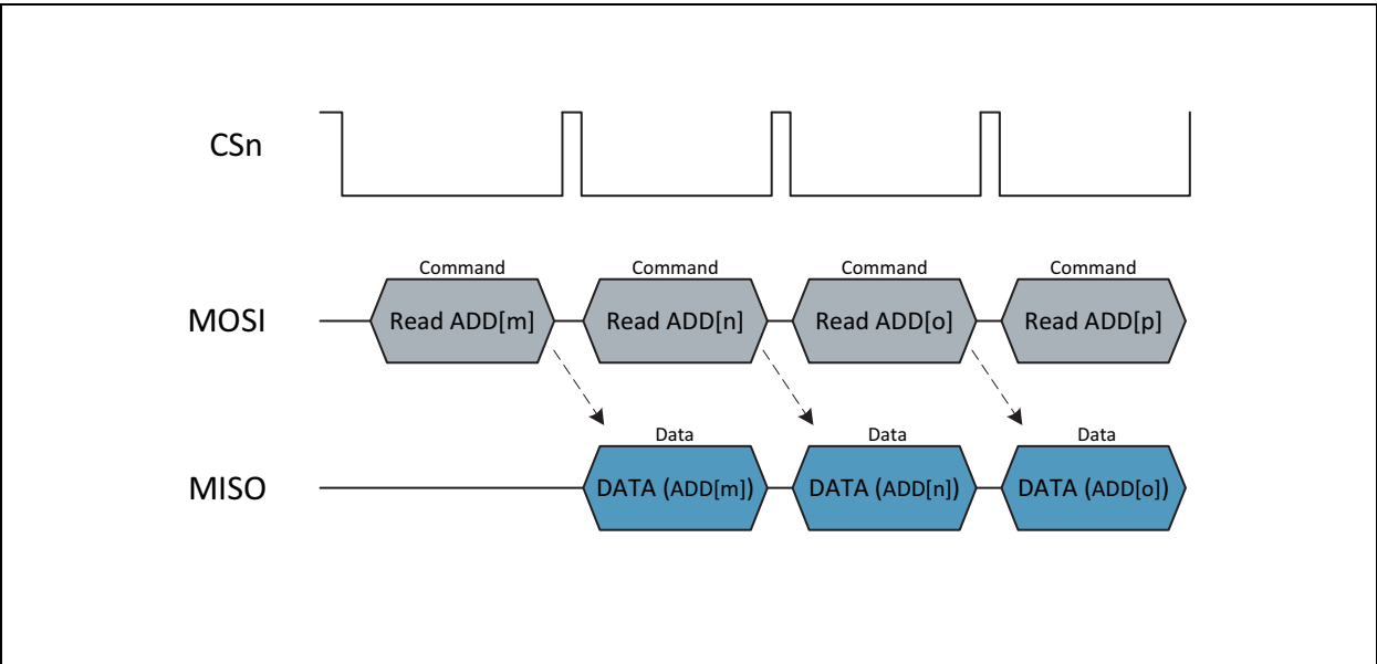
Figure 15: SPI Read
