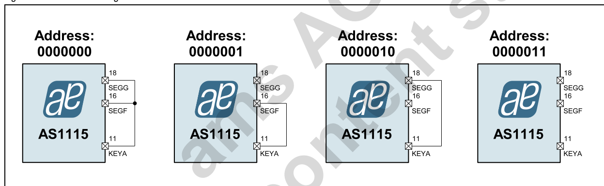
Figure 26. Address Coding
