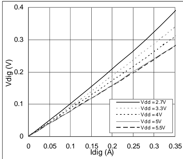
Figure 10. V_{DIGIT} vs. I_{DIGIT}
