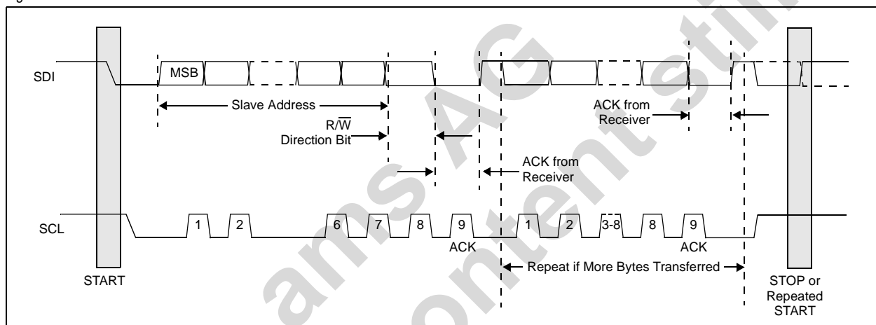
Figure 19. Bus Protocol
