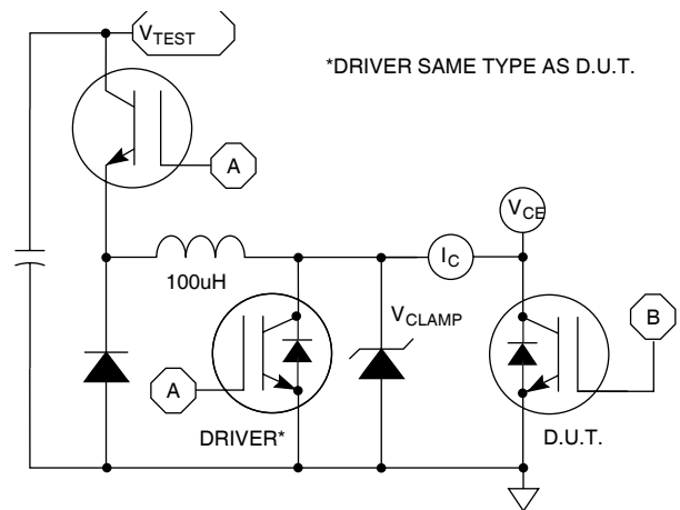
Figure 24, E_{\text{ON1}} Test Circuit
