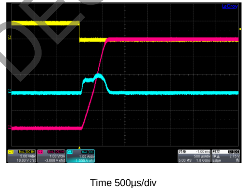
Output Turn Off and Fall Time ( V_{IN} = 5\text{V} , C_{IN} = 1.0\mu\text{F} , C_{OUT} = 470\mu\text{F} , R_L = 3.3\Omega )
