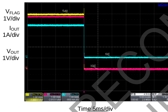
FLAG Response during Over Temperature ( T_A = +125^\circ C )
