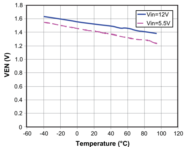
Enable Input Threshold (Rising) vs Temperature
