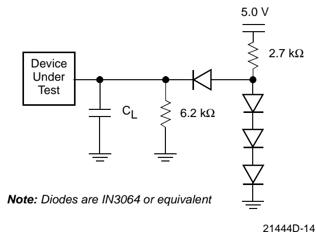
Figure 8. Test Setup
