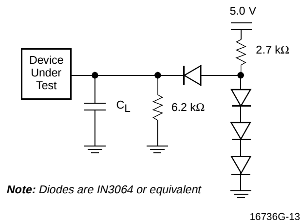
Figure 7. Test Setup
